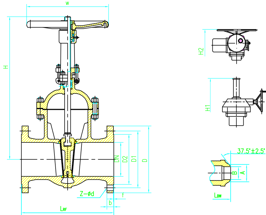
Z40(H, W, Y)-600LB
